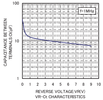
VR- C_t CHARACTERISTICS
