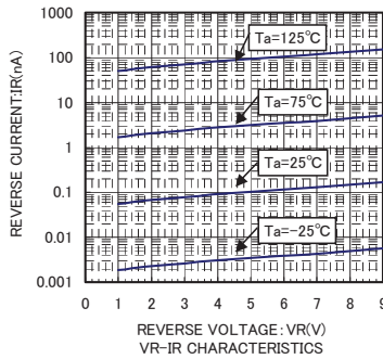
VR- I_R CHARACTERISTICS
