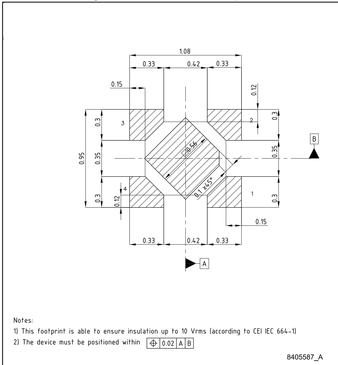
Figure 29: DFN 1x1-4L recommended footprint
