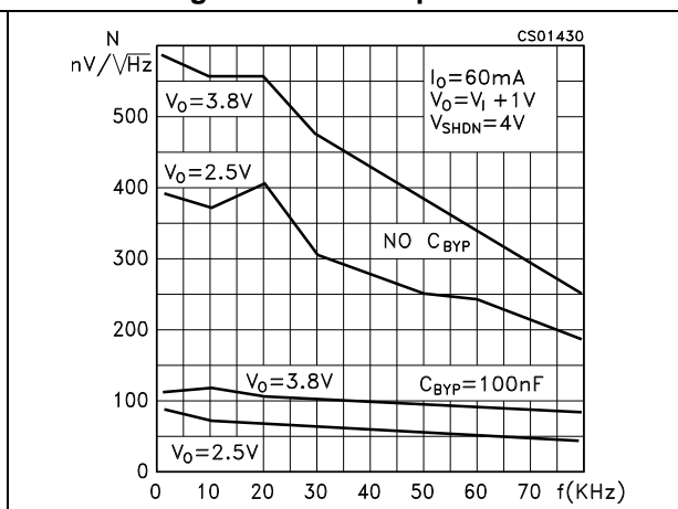
Figure 22. Noise spectrum
