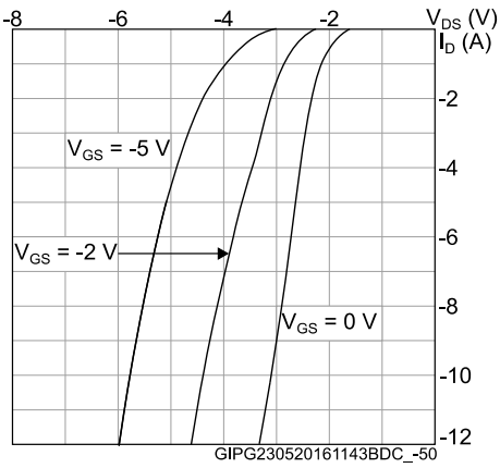
Figure 16: Body diode characteristics ( T_J = -50 \text{ }^\circ\text{C} )
