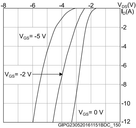
Figure 18: Body diode characteristics ( T_J = 150 \text{ }^\circ\text{C} )
