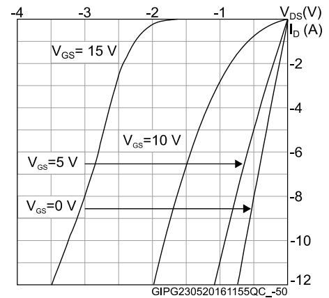
Figure 19: 3rd quadrant characteristics ( T_J = -50 \text{ }^\circ\text{C} )
