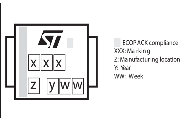
Figure 12. Marking layout (1)
