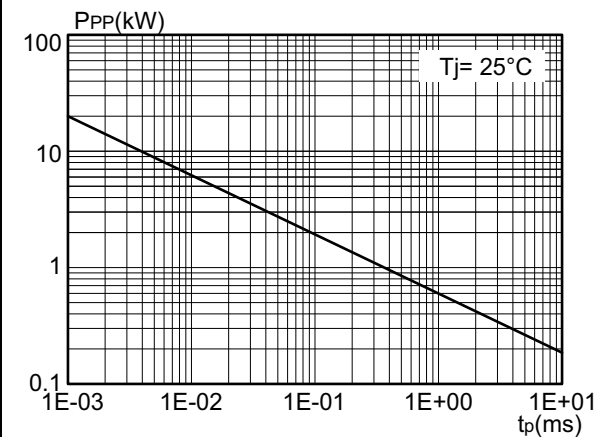
Figure 4. Peak pulse power versus exponential pulse duration (T J initial = 25 °C)
