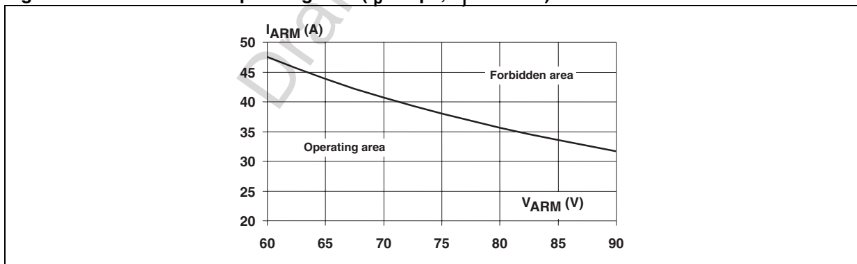
Figure 12. Reverse safe operating area ( t_p < 1\ \mu\text{s} , T_i > 150^\circ\text{C} )
