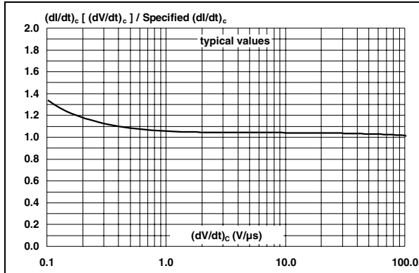
Figure 9. Relative variation of critical rate of decrease of main current (dl/dt)_c versus reapplied (dV/dt)_c
