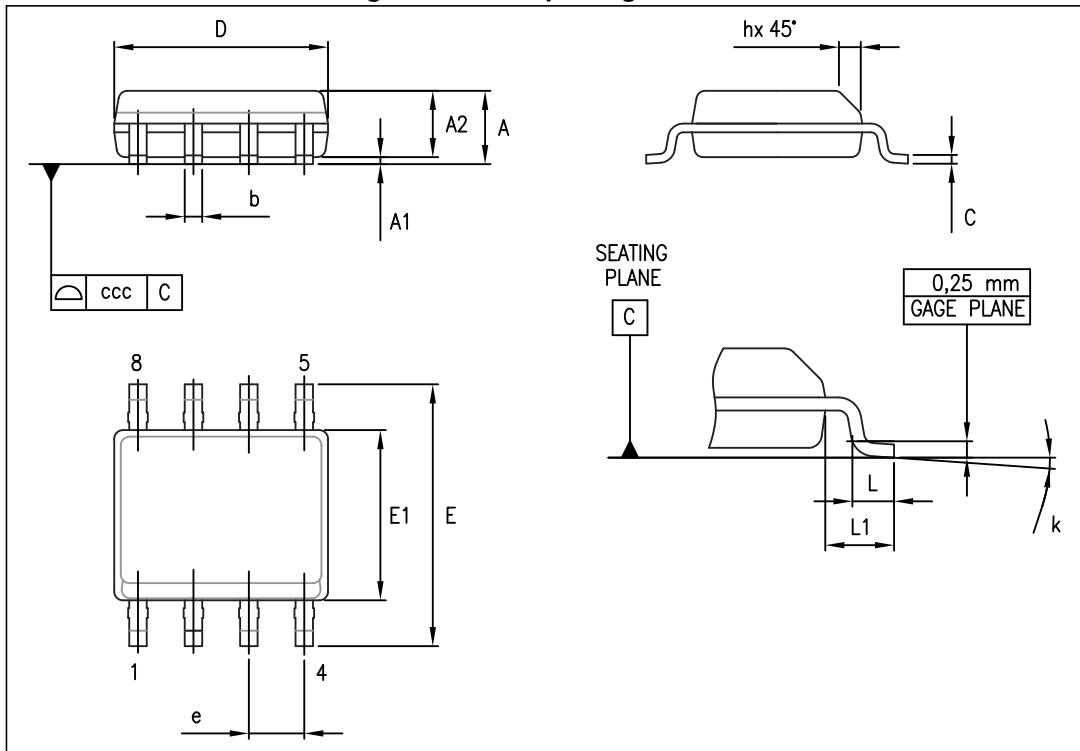
Figure 22. SO-8 package outline
