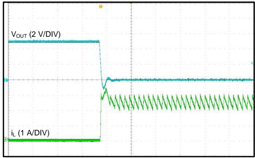
Figure 27. CCM Mode
