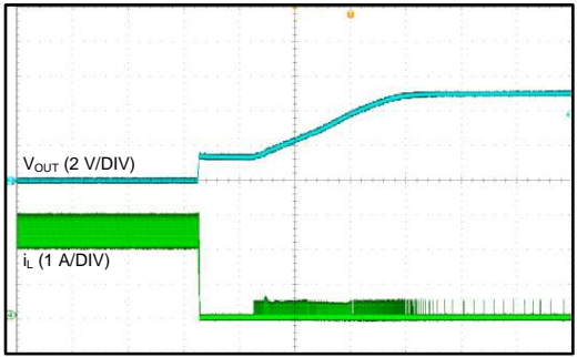
Figure 28. Load Transient
