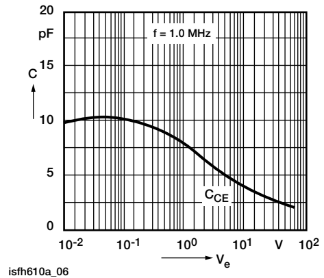
Fig. 6 - Transistor Capacitance (typ.) vs. Collector-Emitter Voltage
