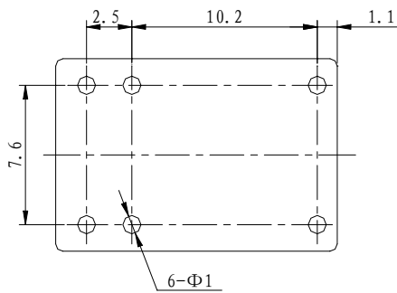
(Bottom View)底视
